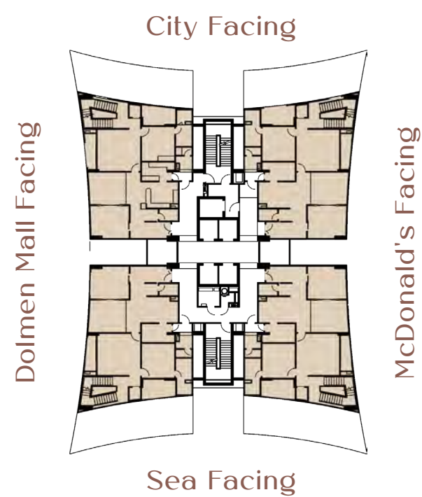
4 BEDROOM SKY VILLAS RESIDENCES (LOWER LEVEL)
